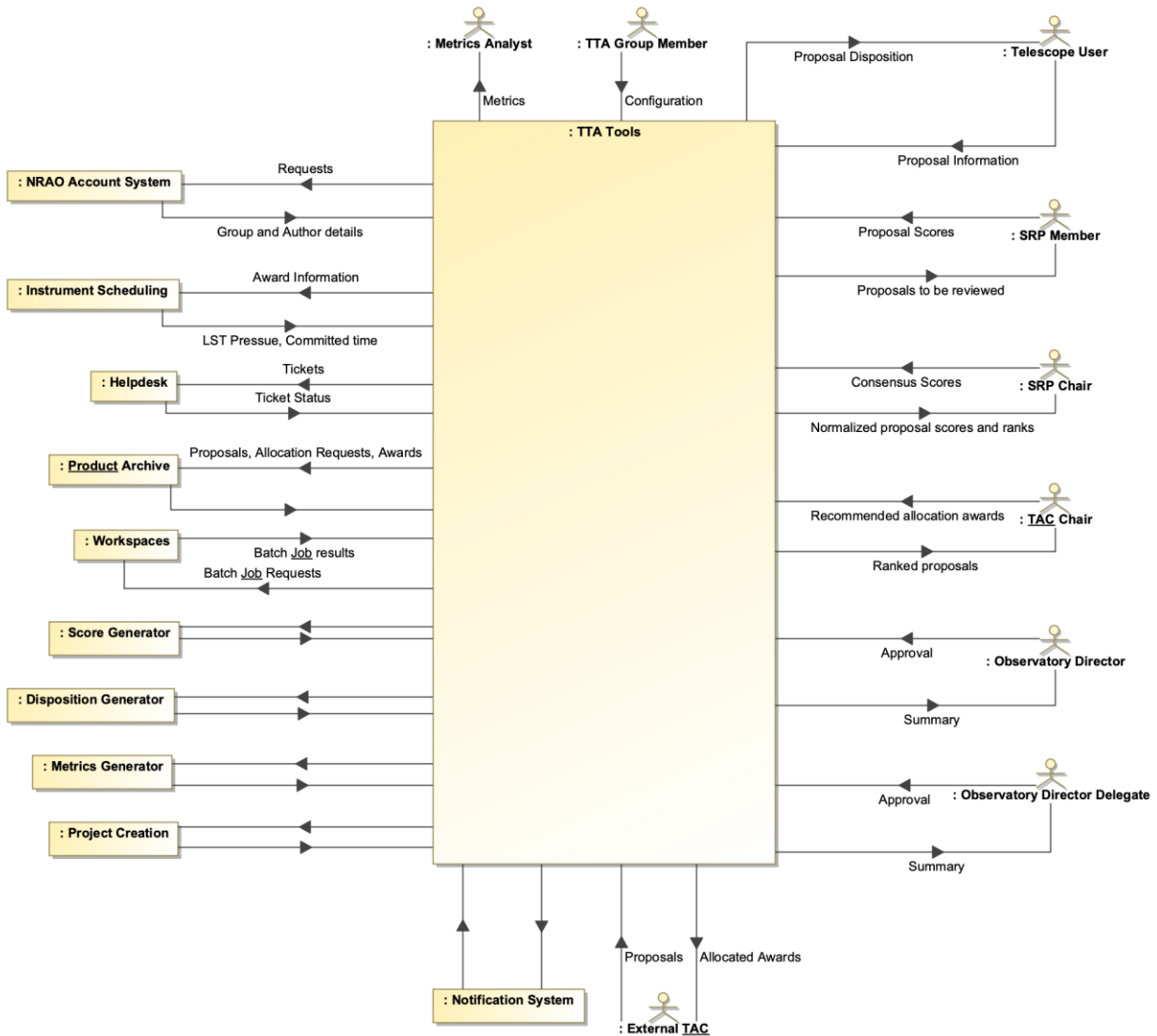
Figure 6 TTA System Context
