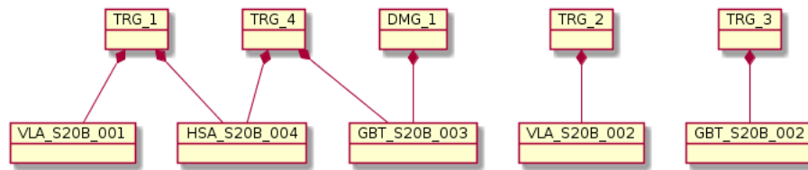
Figure 7: Example of the mapping between feasibility groups and Allocation Requests . Here we show how one FRG (TRG_1) is mapped to two different Allocation Requests , and how one HSA Allocation Request is mapped to two FRGs (TRG_1 and TRG_4).
