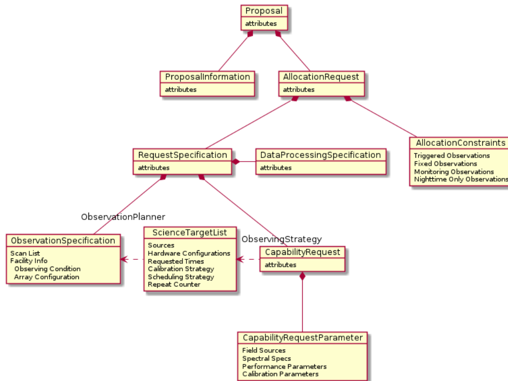
Figure 3: Proposal object diagram. A Proposal is composed of Proposal Information and one or more Allocation Requests . An Allocation Request may have one or more Allocation Constraints . A Capability Request is generated from user input using the available Capabilities for the given Solicitation . The software generates an Observation Specification from the Capability Request via the Science Target List . The Observing Strategy and Observation Planner consist of algorithms and heuristics to make this happen.
