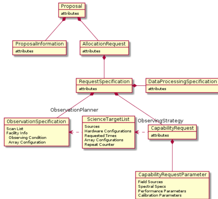
Figure 7: Proposal object diagram. A Proposal is composed of Proposal Information and one or more Allocation Requests . A Capability Request is generated from user input using the available Capabilities for the given Solicitation . The software generates an Observation Specification from the Capability Request via the Science Target List . The Observing Strategy and Observation Planner consist of algorithms and heuristics to make this happen.
